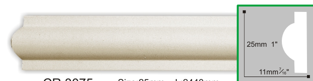
CR 3075 Size:25mm L:2440mm
