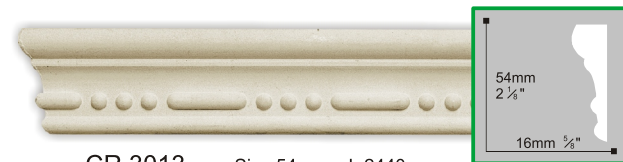
CR 3013 Size:54mm L:2440mm
