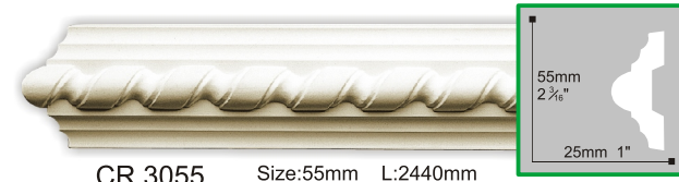
CR 3055 Size:55mm L:2440mm
