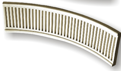
CR 3051(INT) Internal curve :362mm External curve :375mm Height :90mm Thickness :14mm
