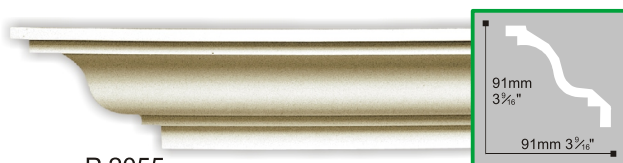
P 2055 Size:129mm L:2440mm
