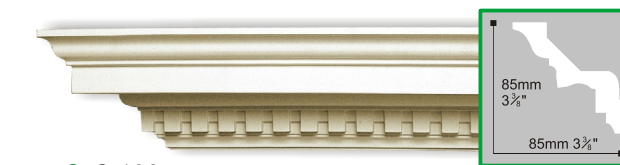
● C 138 Size:119mm L:2440mm
