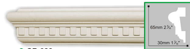
● CR 622 Size:65mm L:2440mm
