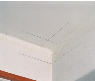
2.Marked on the wall and ceiling using the cornices to prepare for corner joints.
