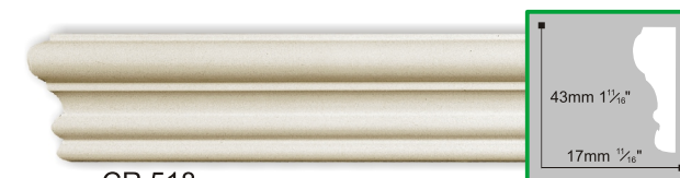
CR 518 Size:43mm L:2440mm
